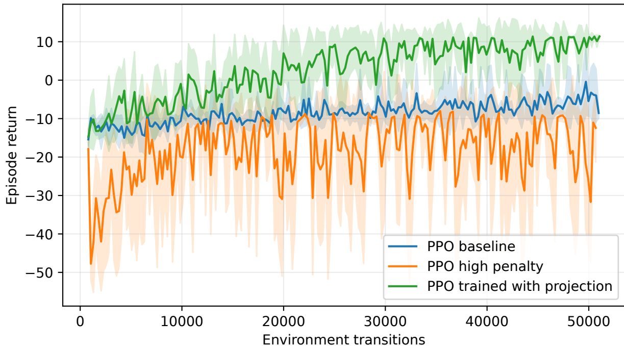
Episode return Not directly comparable: collision penalty 50 (PPO high penalty) vs 10 (others)
