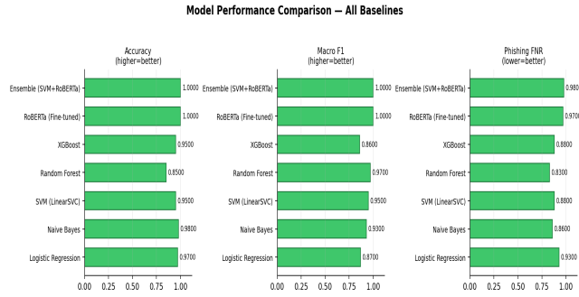
Fig. 8. Final model comparison: accuracy, macro F1 and phishing false-negative rate across all classifiers.
