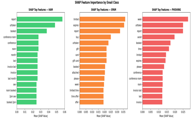
Fig. 4. SHAP feature importance bar charts for all three classes (ham, spam, phishing).
