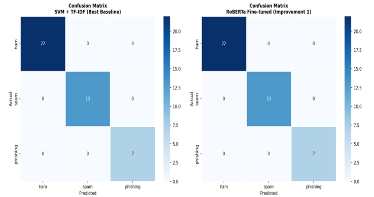
Fig. 6. Confusion matrices for the best-performing classical baseline (SVM + TF-IDF) and the fine-tuned RoBERTa model.
