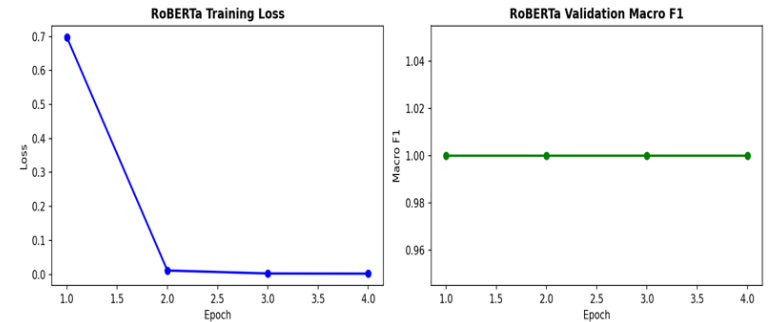
Fig. 2. RoBERTa fine-tuning training loss and validation macro F1 across epochs.
