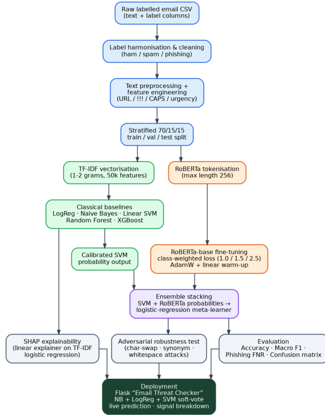
Fig.0. Overall system pipeline: data preparation, the parallel classical and transformer modelling tracks, ensemble stacking, evaluation/explainability/robustness testing, and deployment
