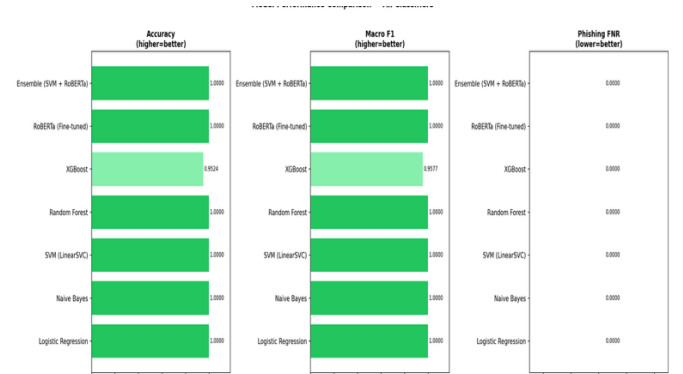
Fig. 9. Final model comparison: accuracy, macro F1 and phishing false-negative rate across all classifiers.
