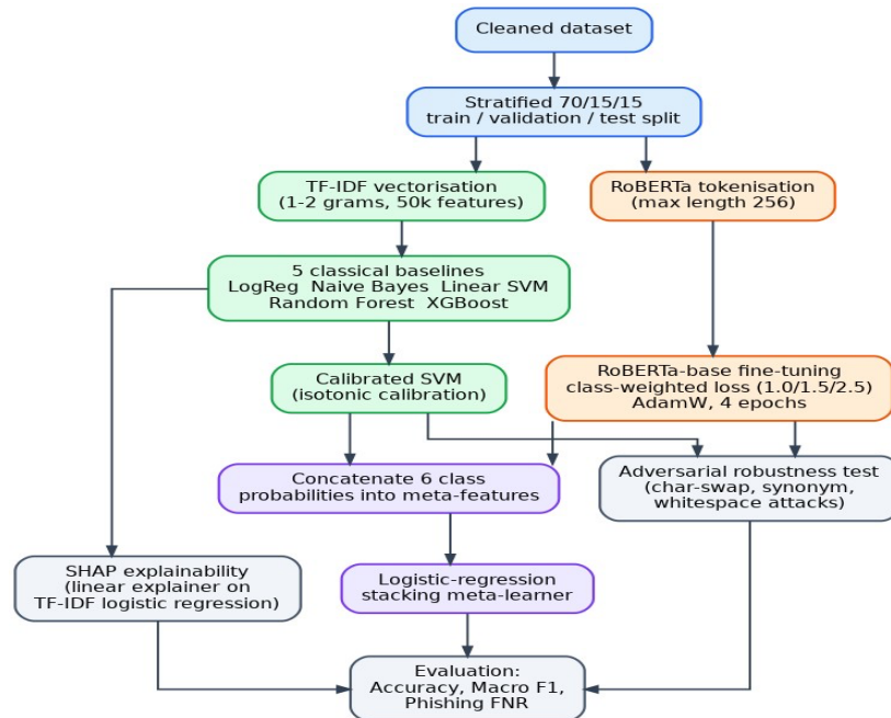
Figure 2. Model training and ensemble flowchart: the parallel TF-IDF/classical and RoBERTa/transformer tracks, their convergence into the stacked ensemble, and the SHAP and adversarial-robustness evaluation branches.
