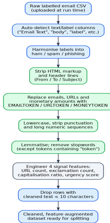
Figure 1. Data preprocessing flowchart: from raw uploaded CSV through label harmonisation, text cleaning, tokenisation and feature engineering, to a cleaned dataset ready for splitting.
