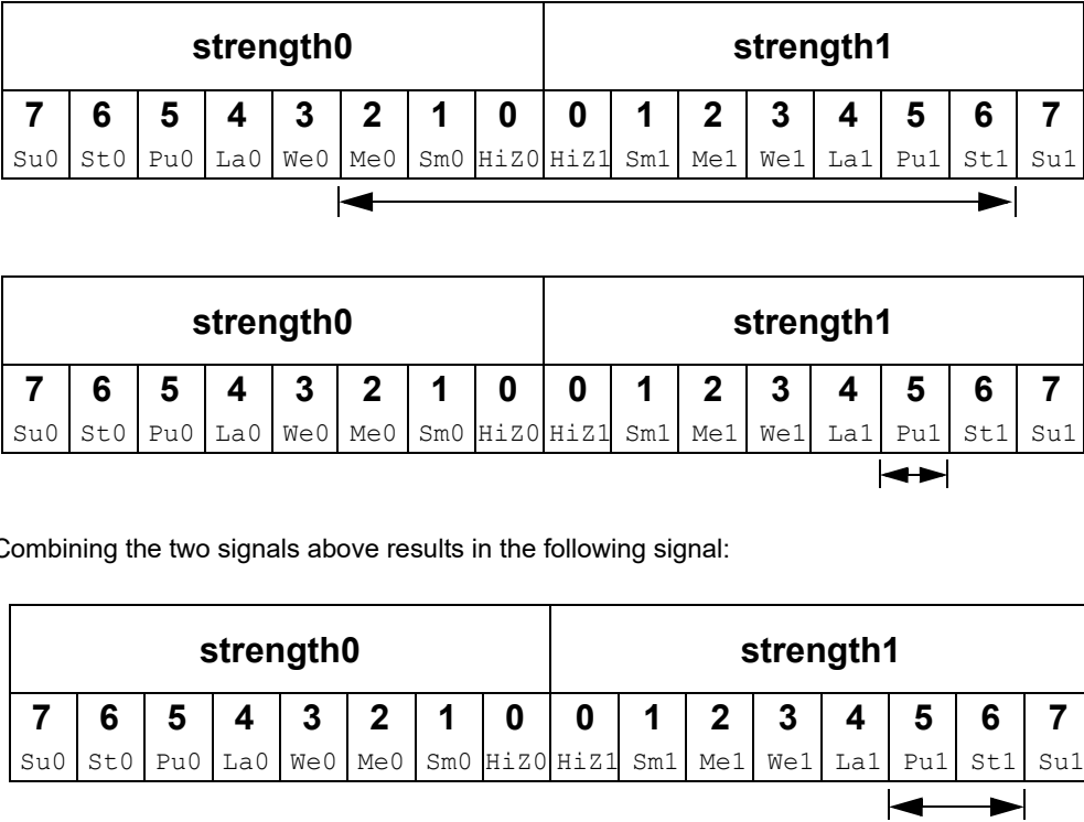
Figure 28-21—Result showing a range and the elimination of strength levels of two values
