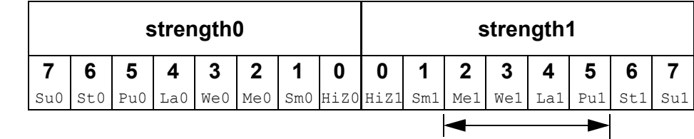
Figure 28-22—Result showing a range and the elimination of strength levels of one value
