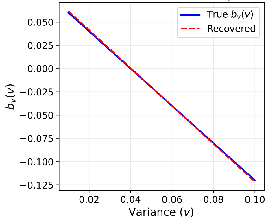
Variance Drift Recovery
