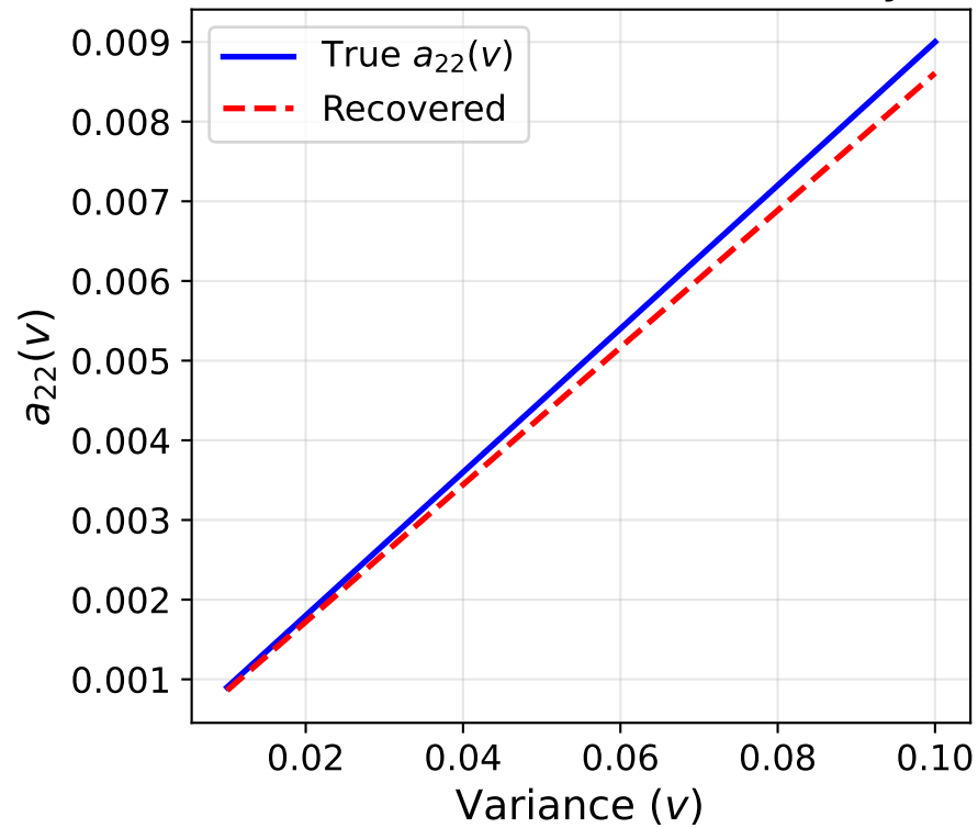
Variance Diffusion Recovery
