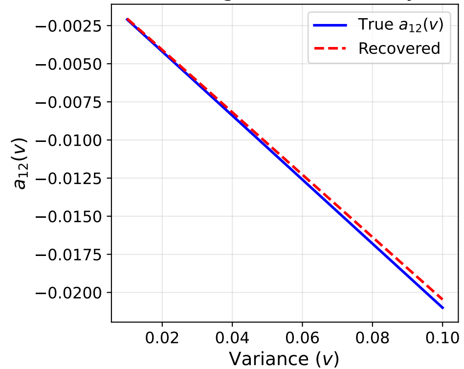
Leverage Effect Recovery
