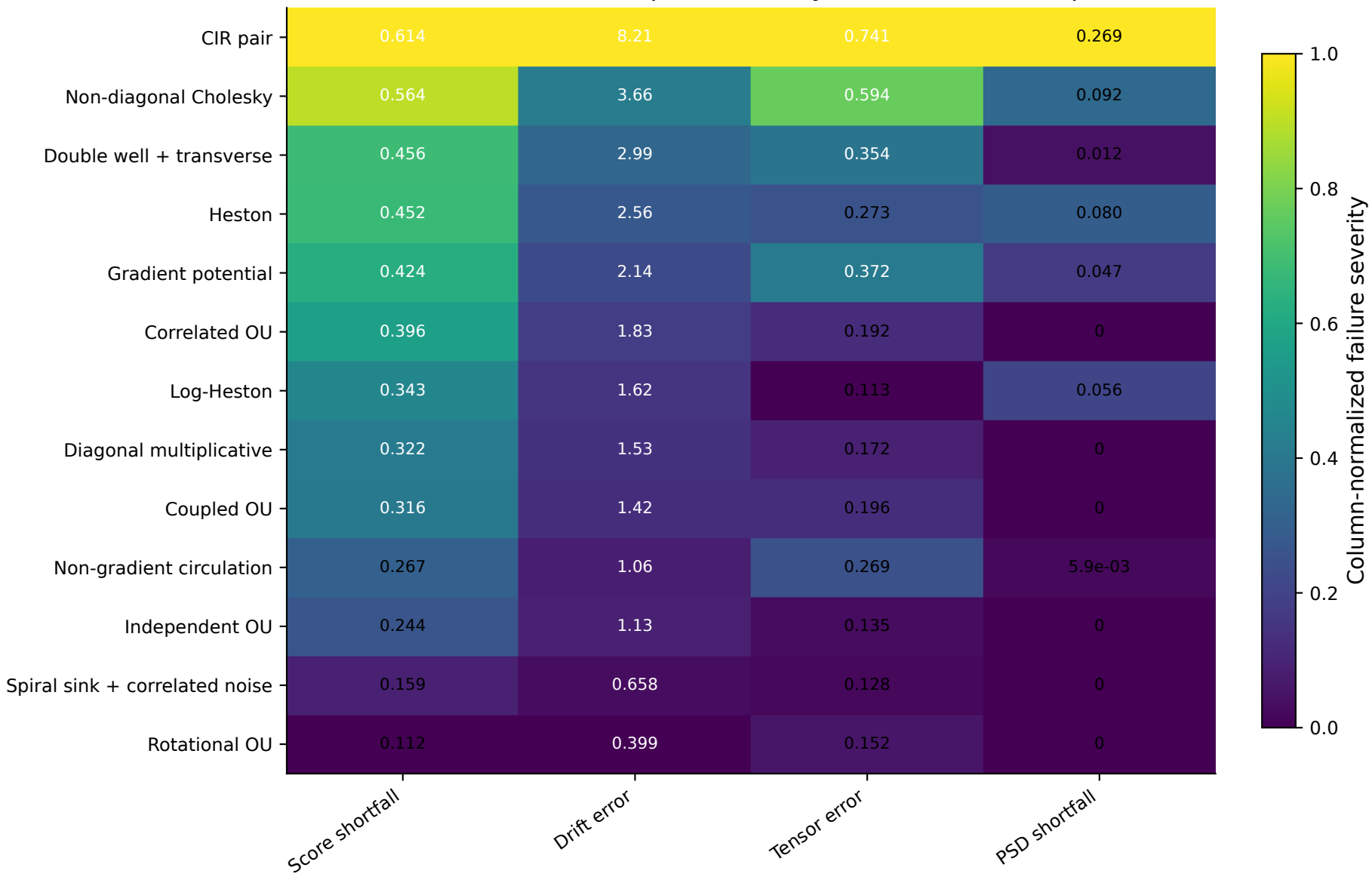
Naive 1D weak-form port on 2D systems: failure hotspots
