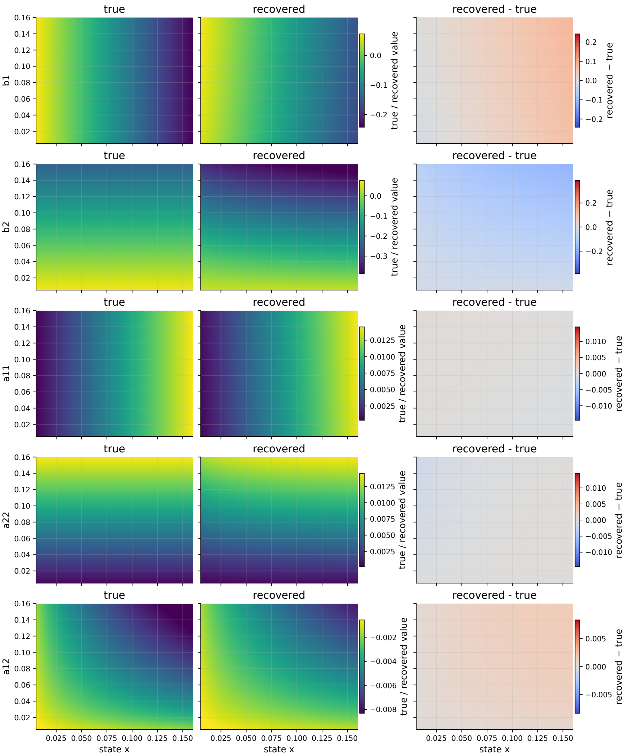
Recovered vs.\ true generator fields: CIR pair
