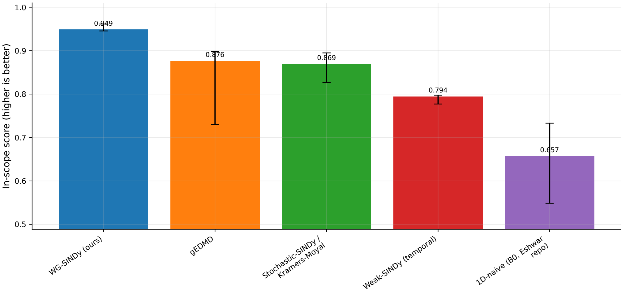
Head-to-head: one aggregated bar per method
