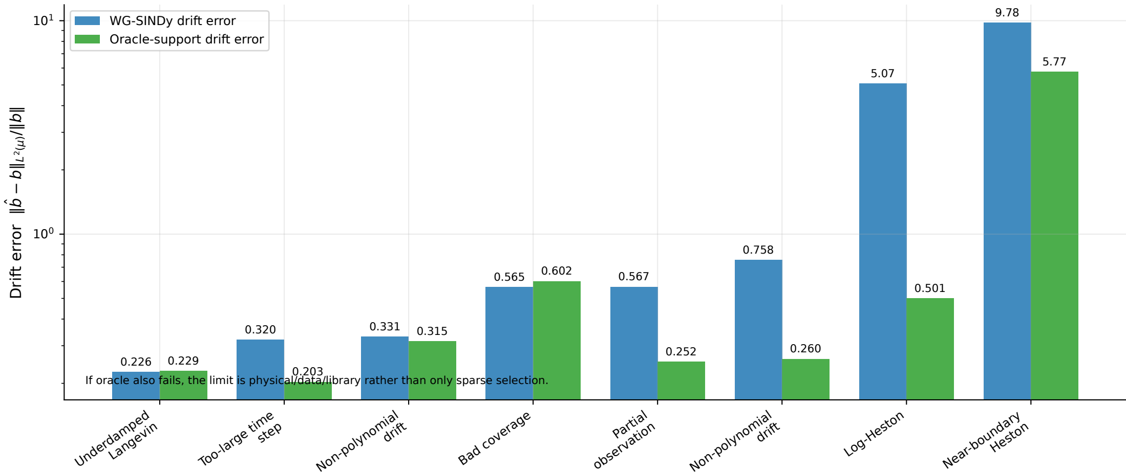
Honest nulls: estimator error vs oracle headroom
