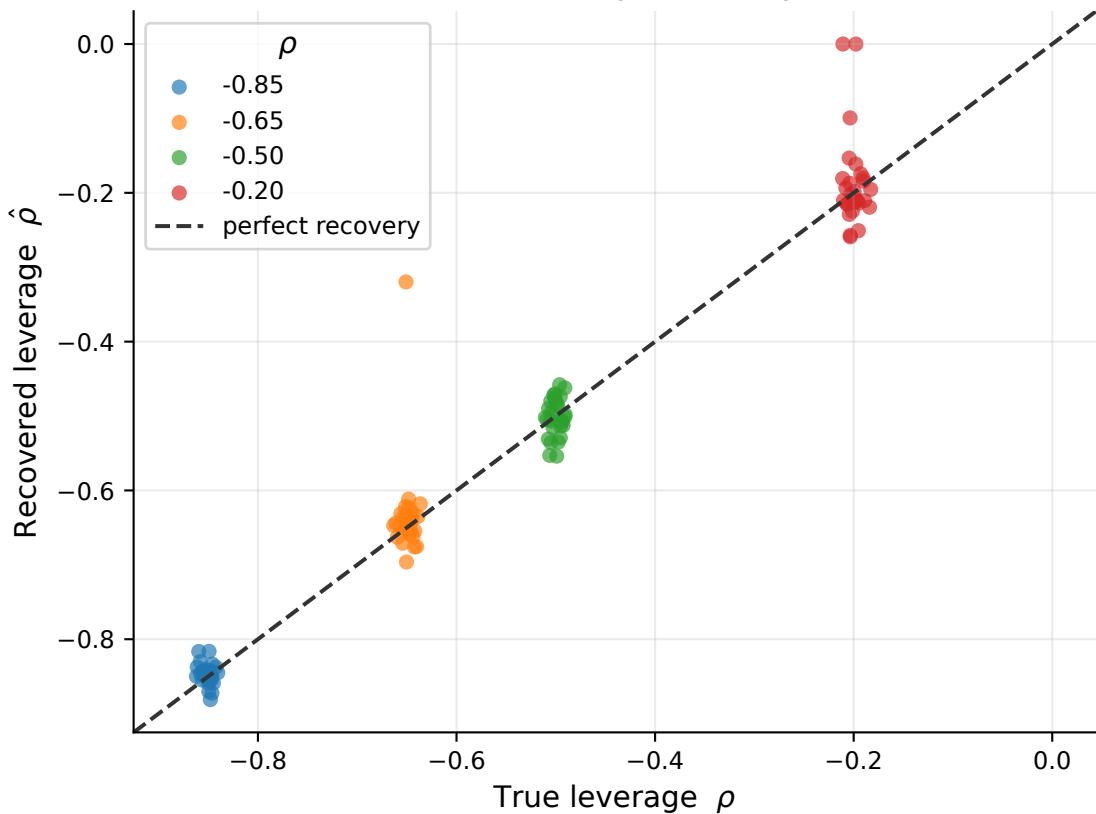
Recovered \hat{\rho} vs true \rho
