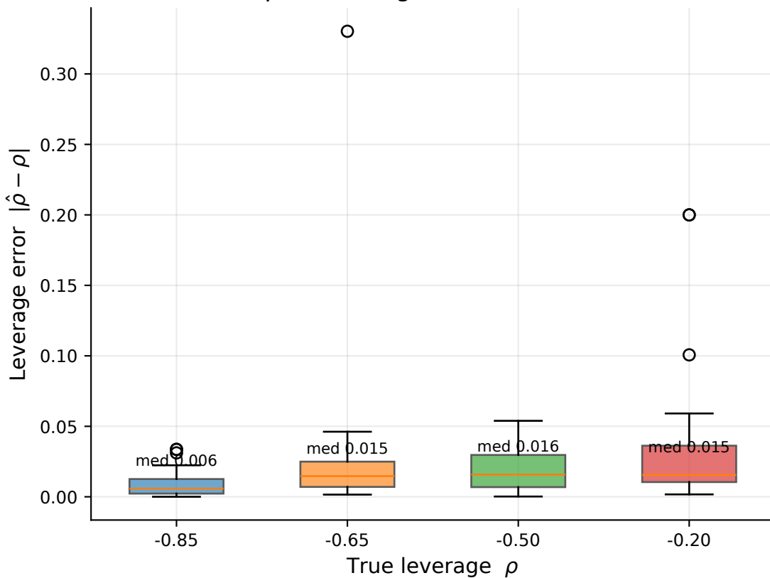
Grouped leverage error across seeds
