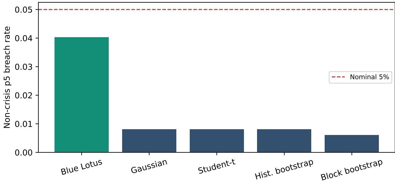
Calm-market tail calibration by model
