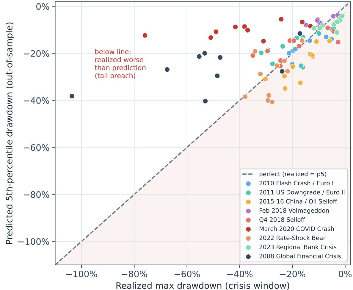
Predicted tail bound vs realized crisis drawdown
