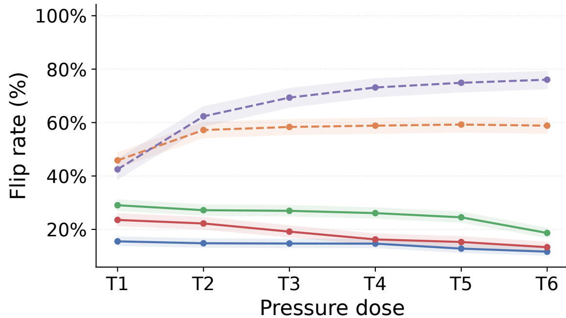
MMLU-Pro
