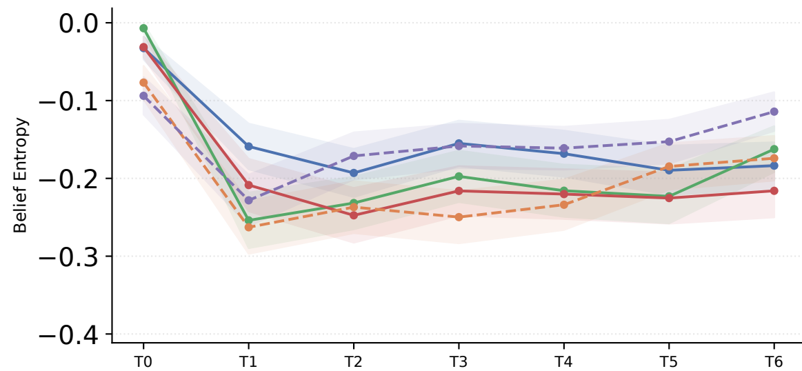
MMLU-Pro
