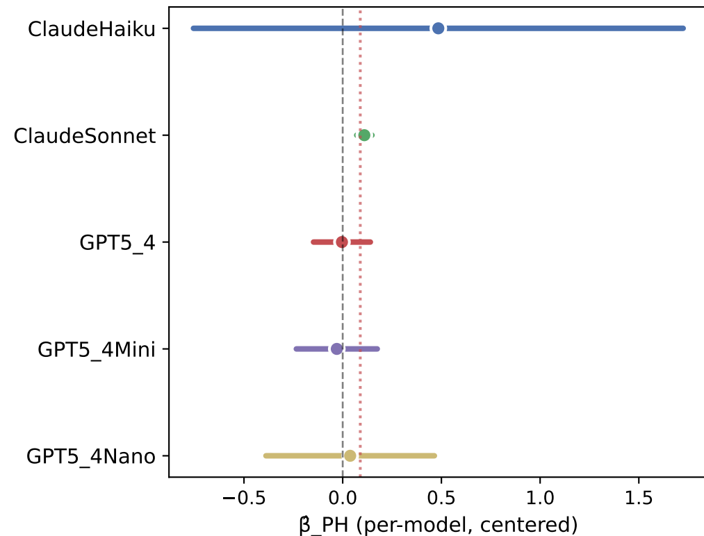
Per-model interaction (95% CI)
