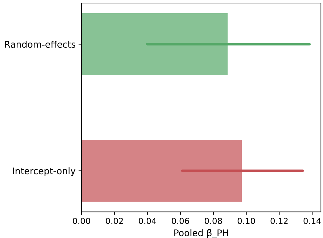
Pooled estimates (wider CI = more honest)
