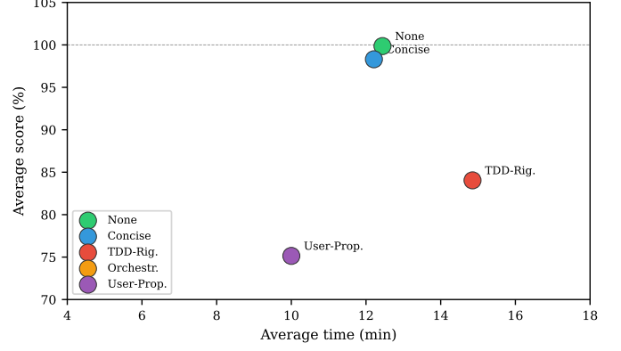
Fig. 6. Speed vs. accuracy trade-off (Round 2)
