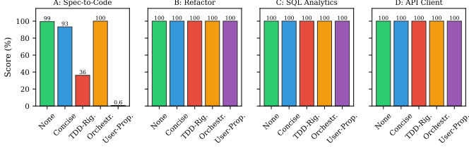
Fig. 4. Round 2 accuracy across all four tracks. Only Track A breaks saturation.
