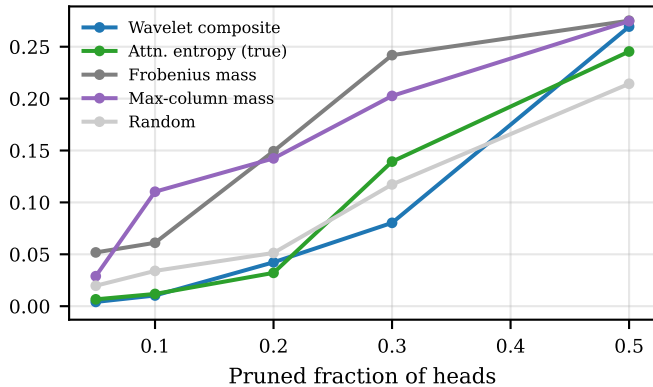
Sentence-embedding cosine drop
