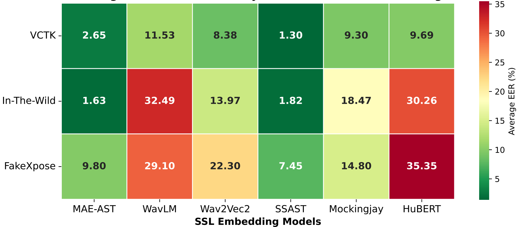
Average EER Performance by Dataset and SSL Embedding
