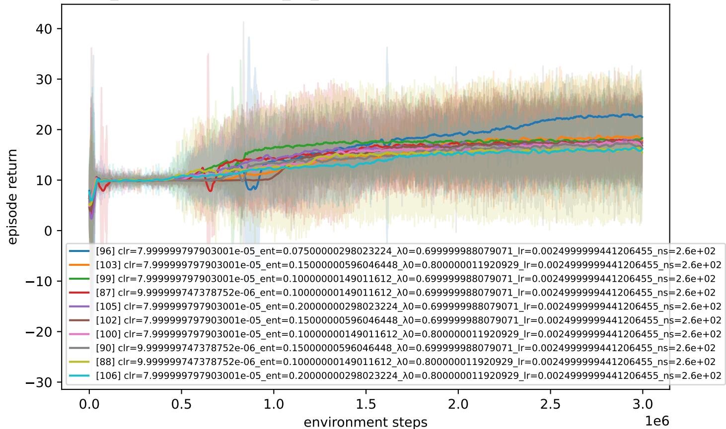
leg_qurnn — rocksample_11_11 (combined 4 studies) — top 10 of 144
