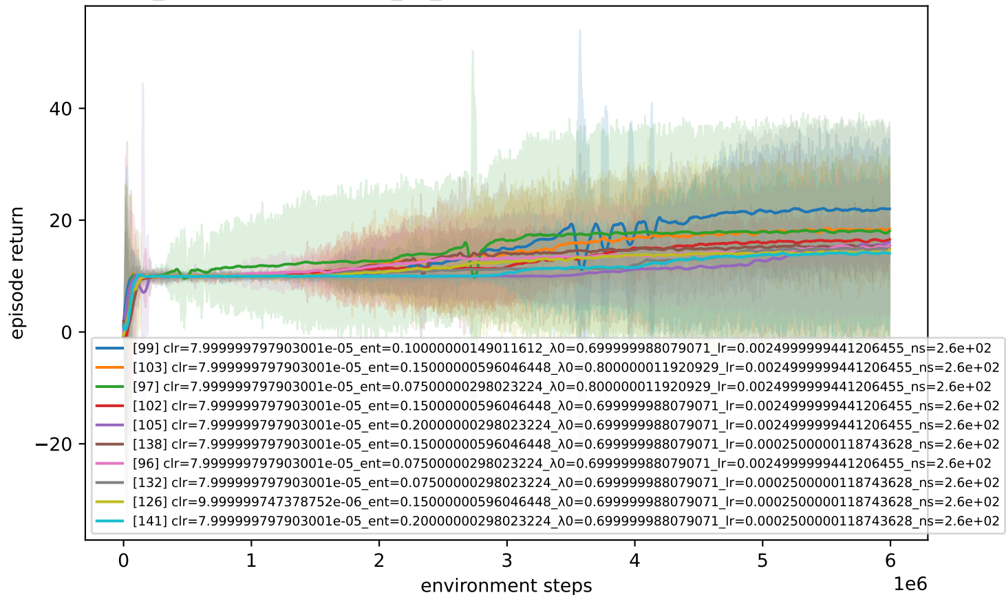
leg_qurnn — rocksample_15_15 (combined 4 studies) — top 10 of 144
