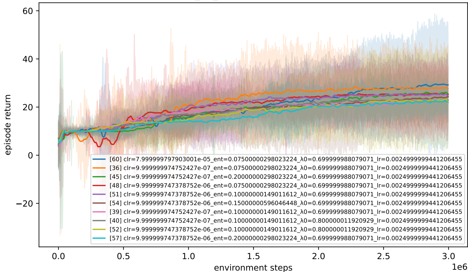
legurnn — rocksample_11_11 (combined 3 studies) — top 10 of 108
