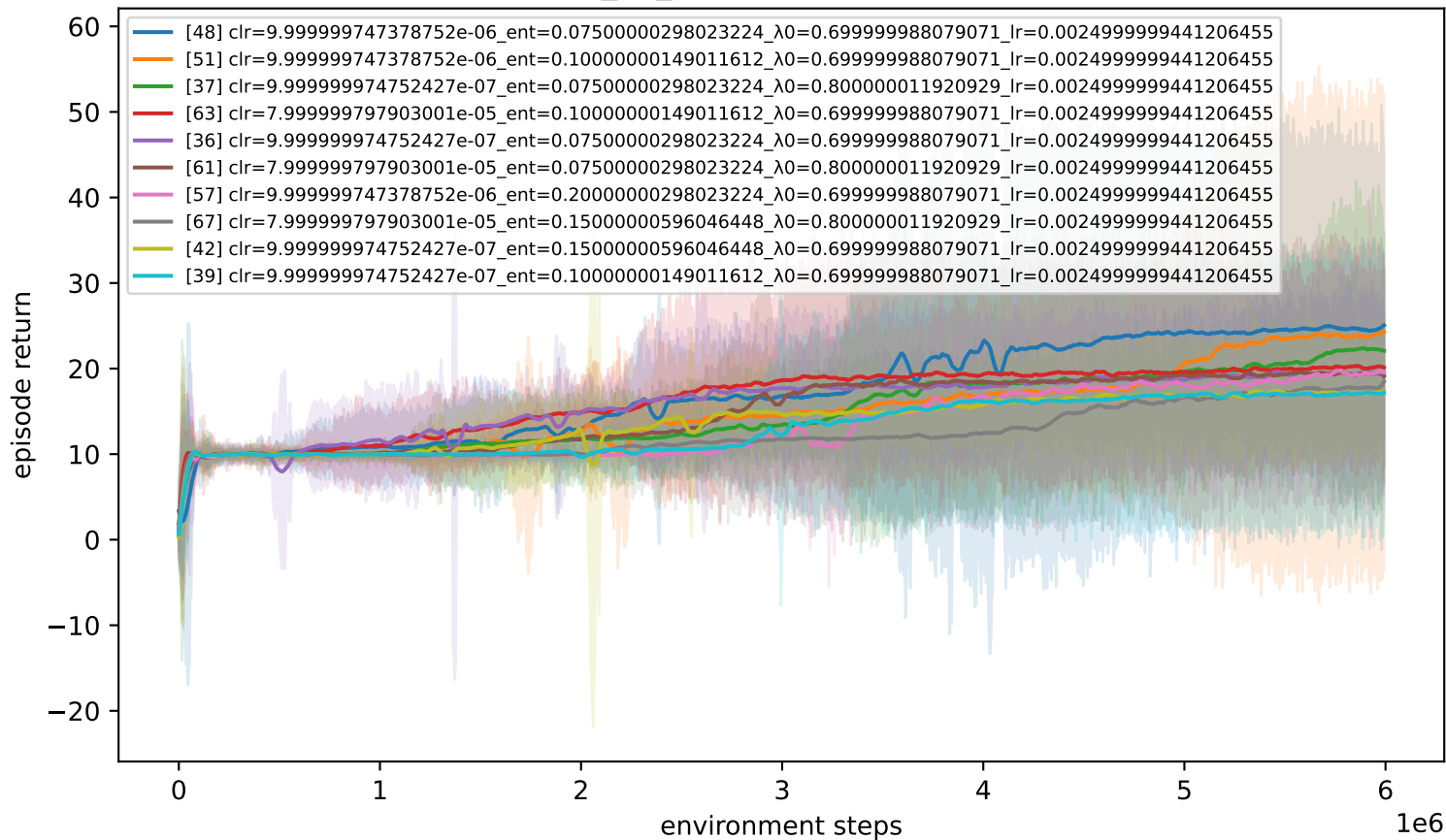
legurnn — rocksample_15_15 (combined 3 studies) — top 10 of 108
