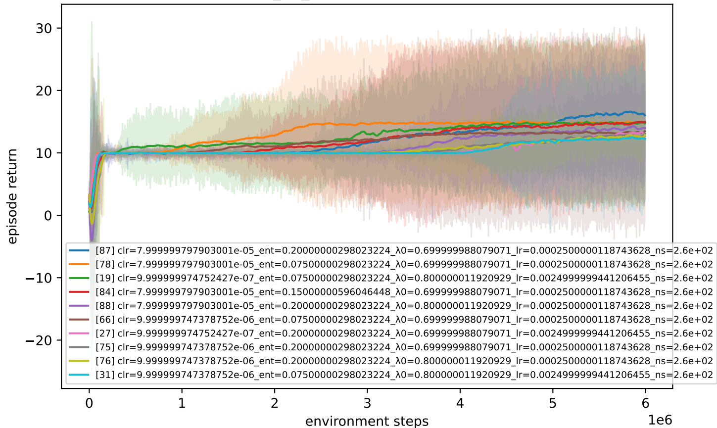
qurnn — rocksample_15_15 (combined 3 studies) — top 10 of 90
