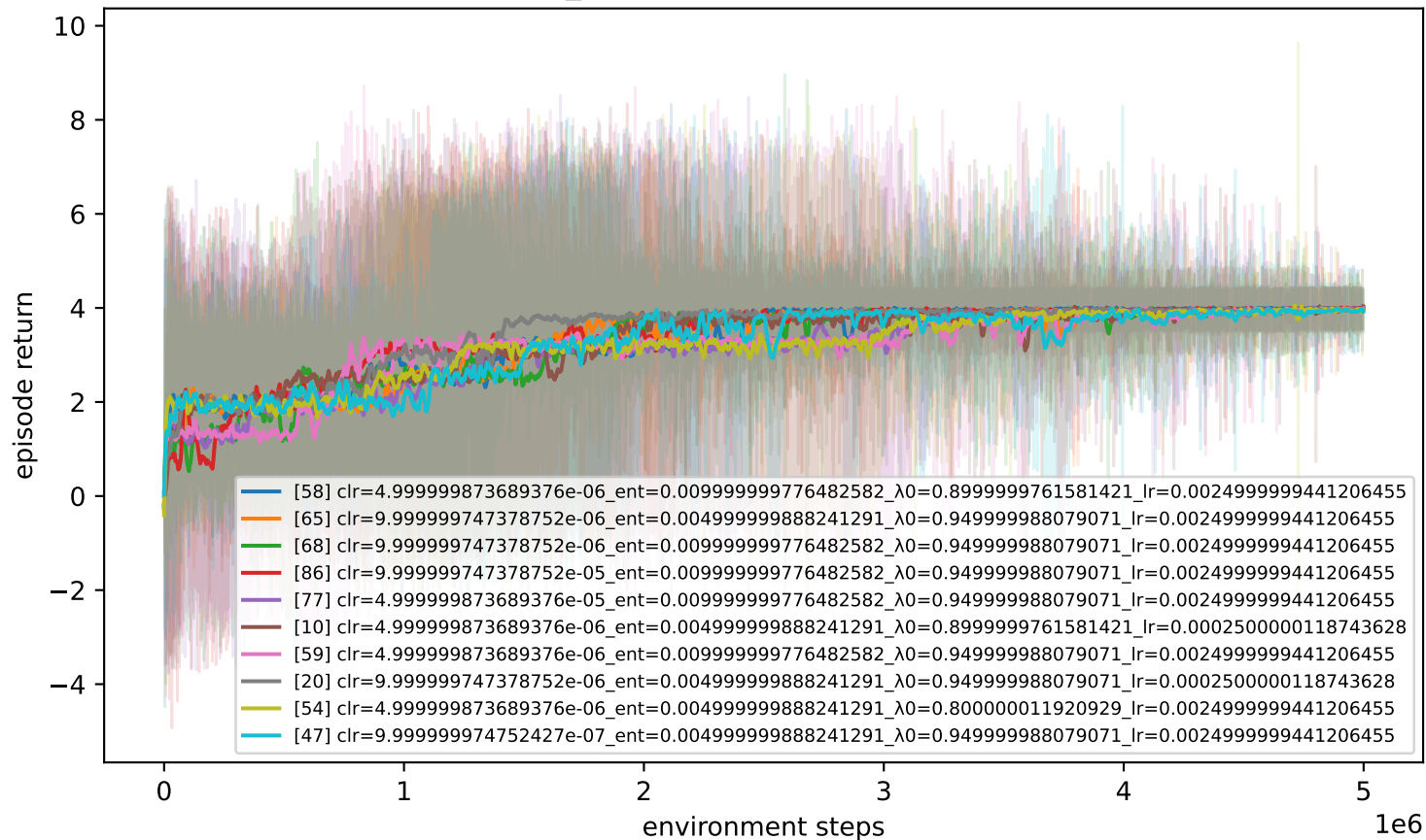
qurnn — tmaze_75 (combined 2 studies) — top 10 of 90
