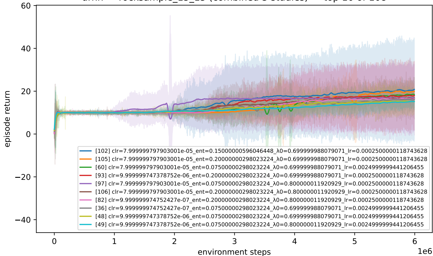
urnn — rocksample_15_15 (combined 3 studies) — top 10 of 108
