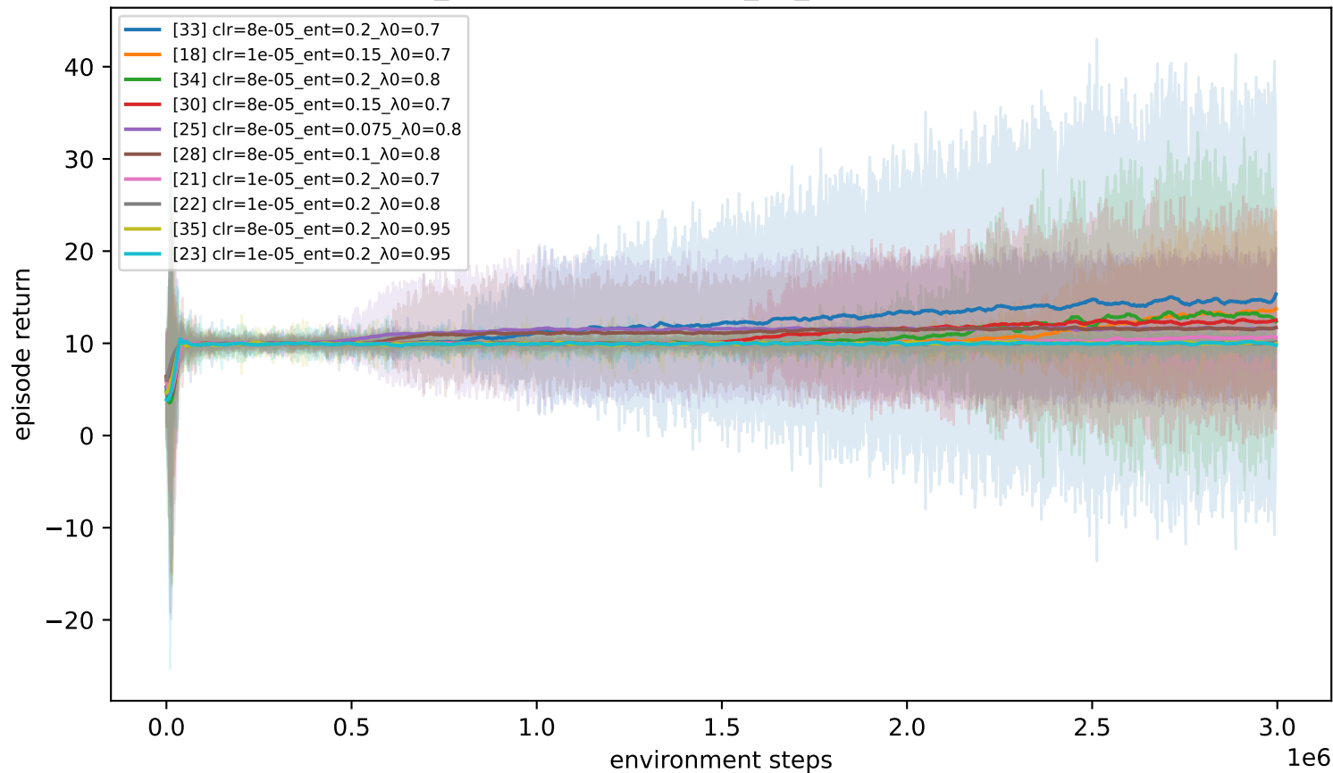
leg_qurnn — rocksample_11_11 (top 10 of 36)
