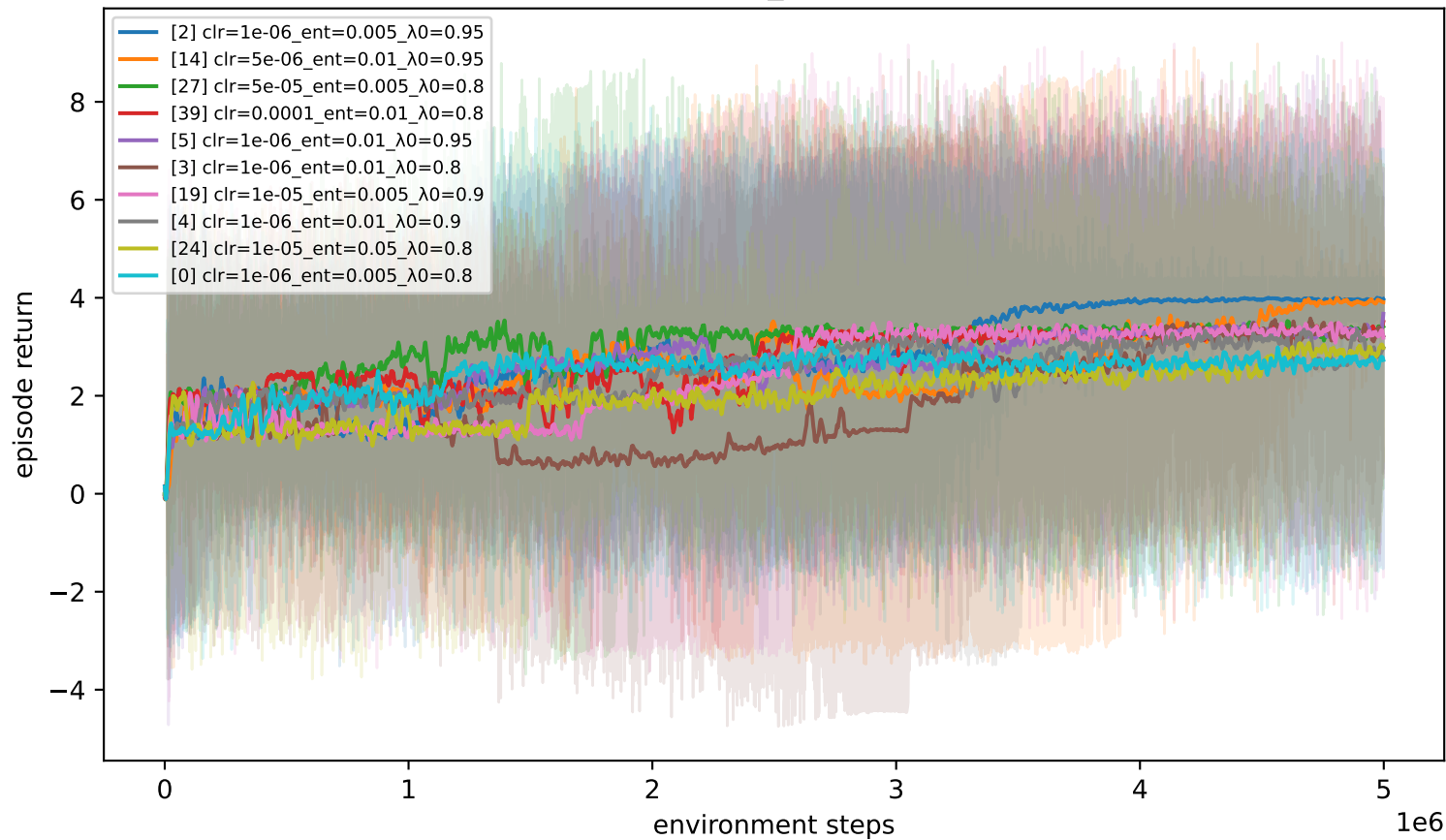
legurnn — tmaze_75 (top 10 of 45)
