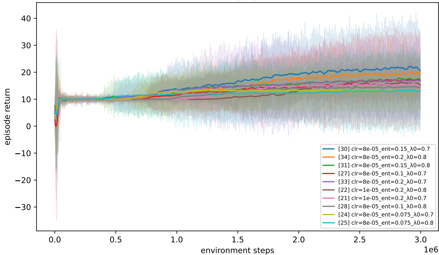
qurnn — rocksample_11_11 (top 10 of 36)
