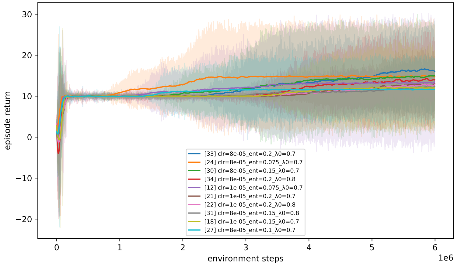
qurnn — rocksample_15_15 (top 10 of 36)
