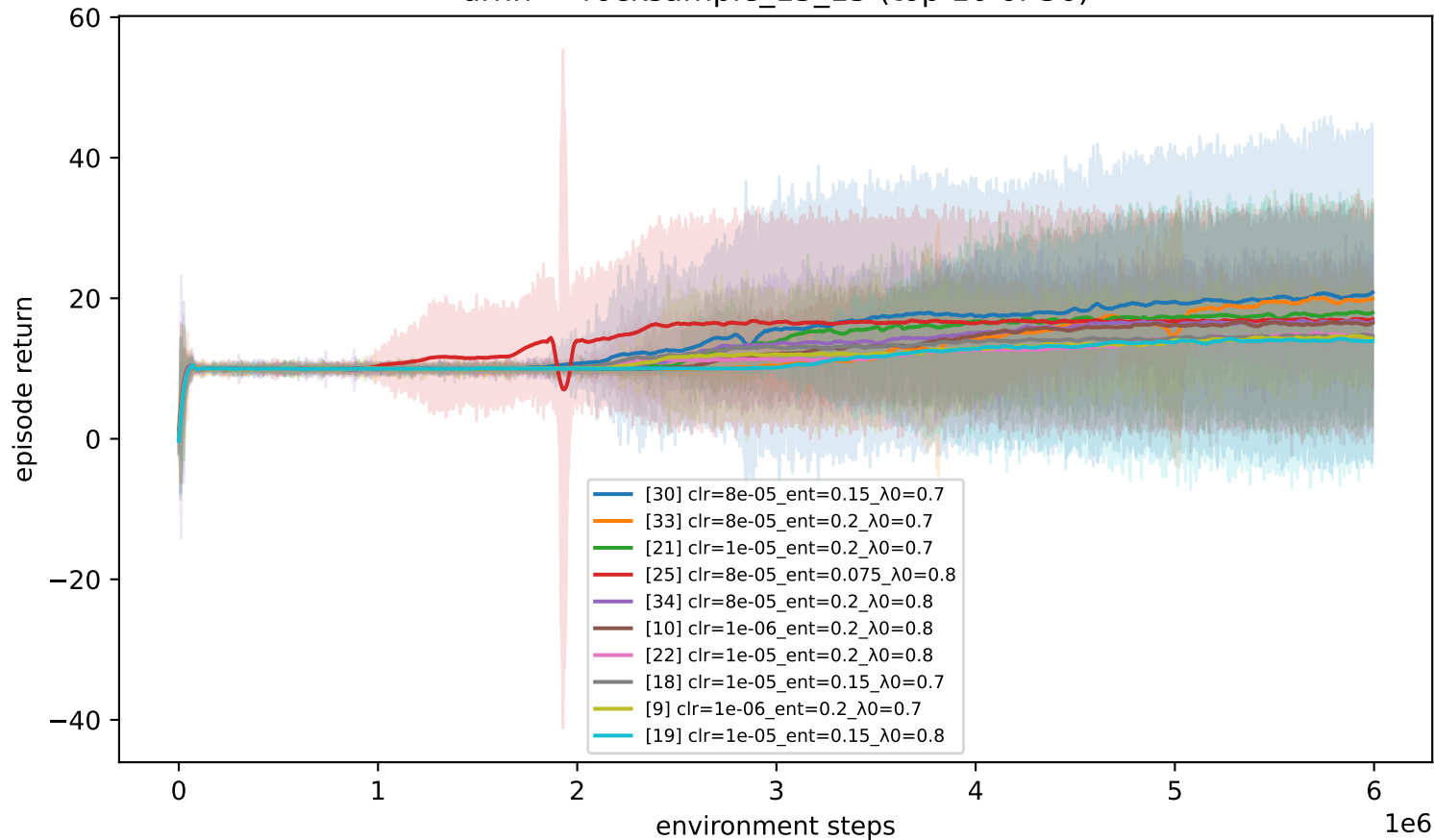
urnn — rocksample_15_15 (top 10 of 36)
