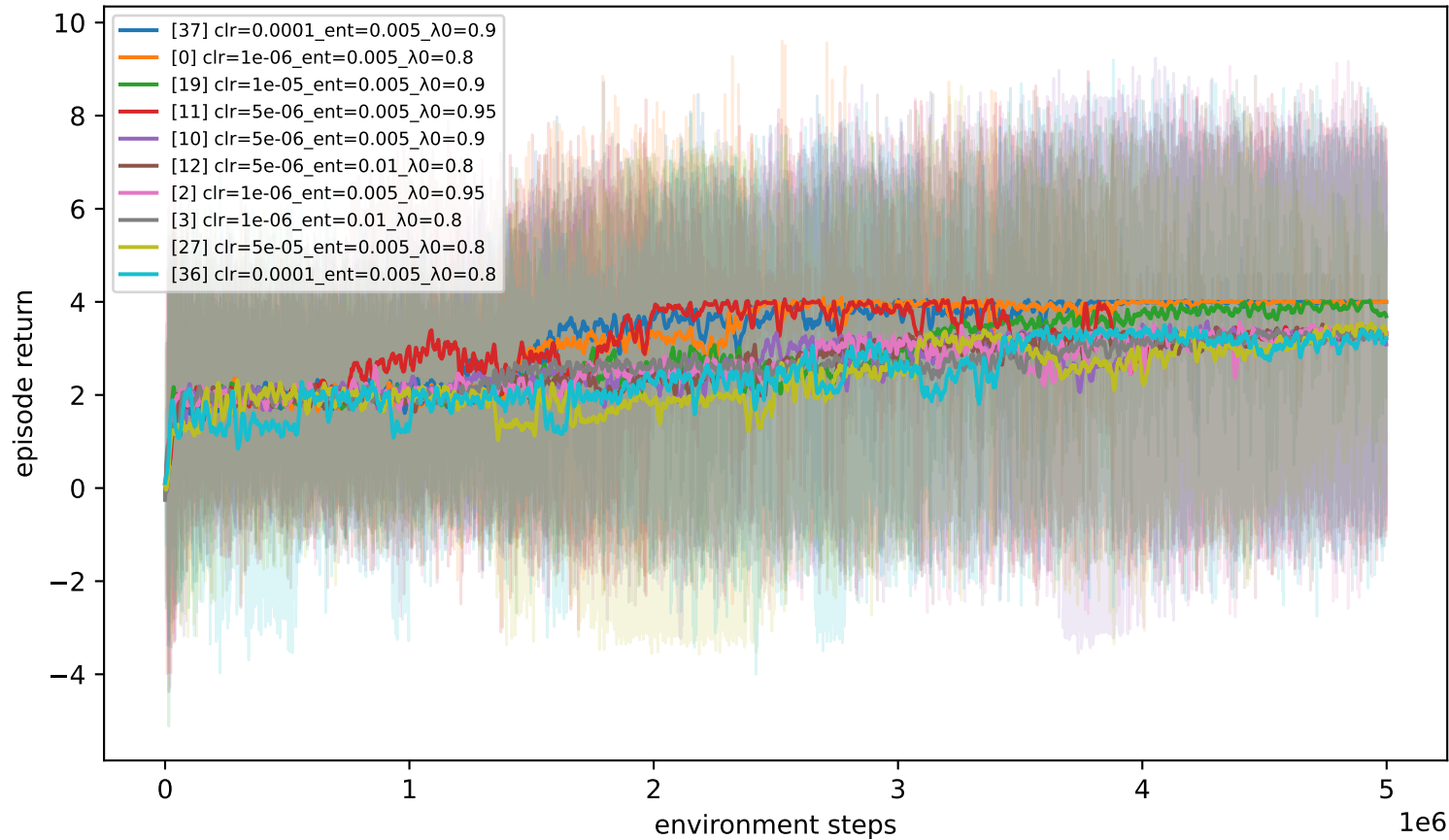
urnn — tmaze_100 (top 10 of 45)
