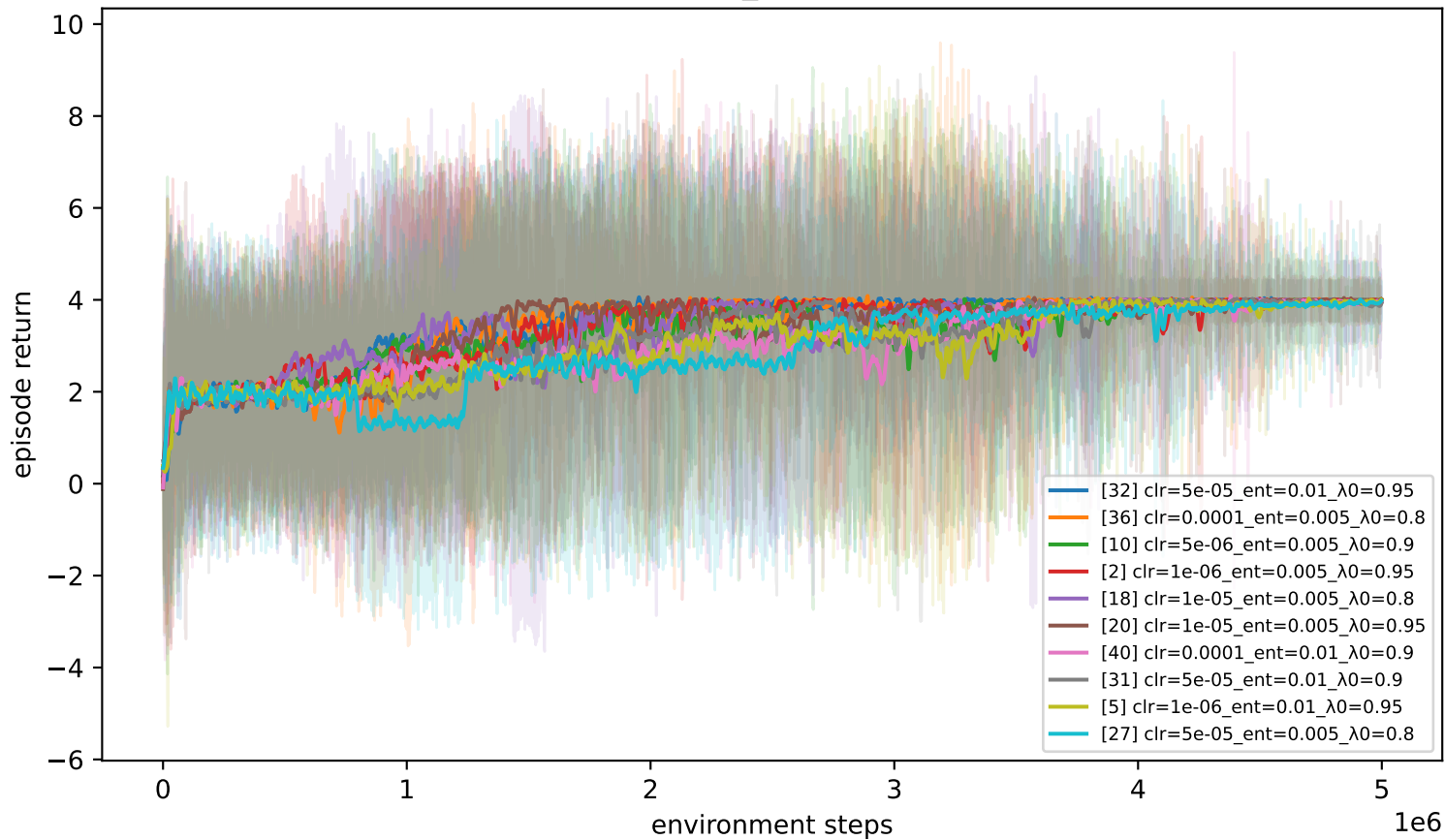
urnn — tmaze_75 (top 10 of 45)
