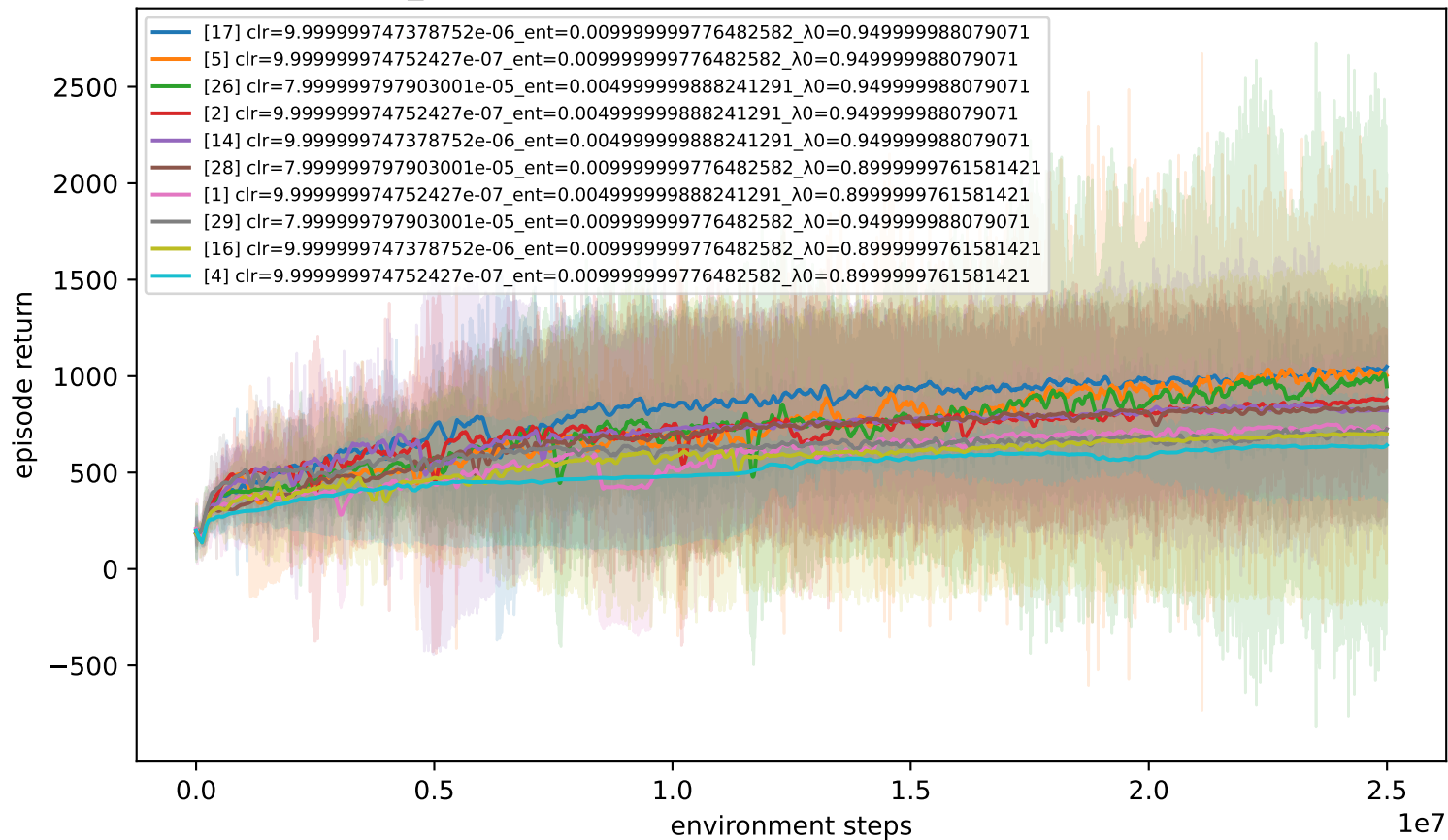
eunn_2 — Walker-V-v0 (combined 1 studies) — top 10 of 36
