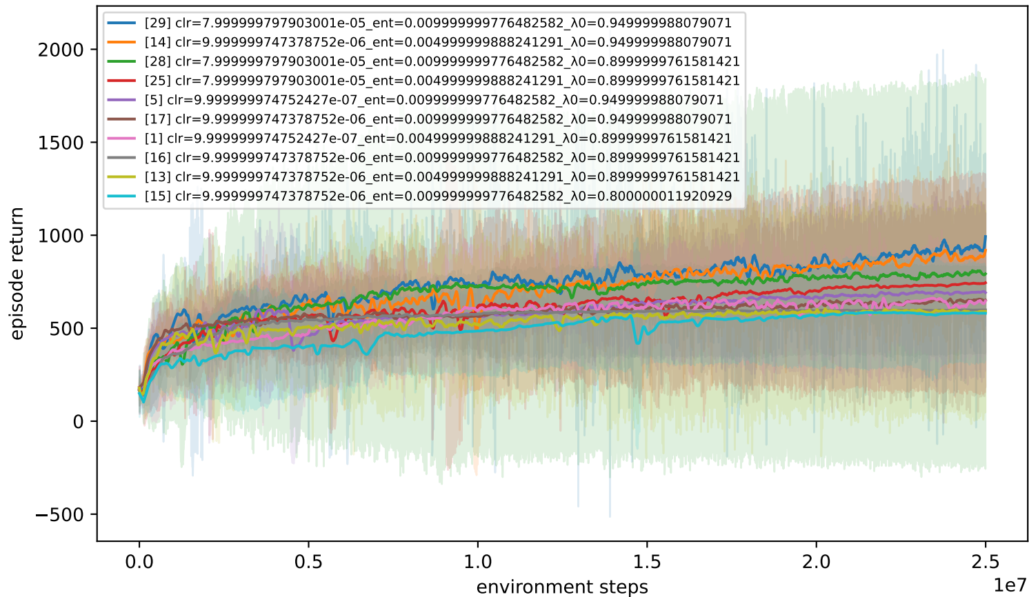
legurnn — Walker-V-v0 (combined 1 studies) — top 10 of 36
