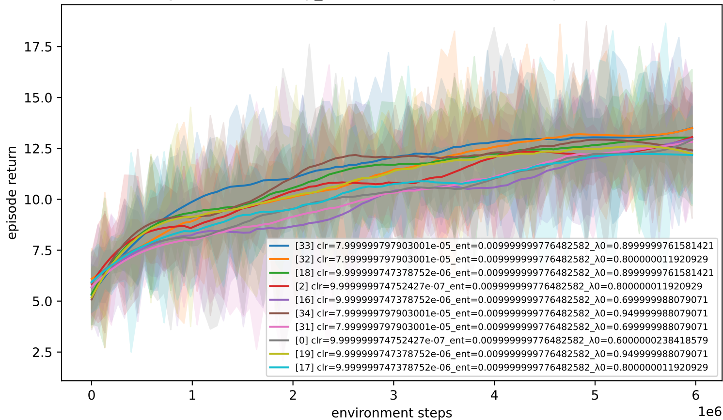
legurnn — battleship_10 (combined 1 studies) — top 10 of 45
