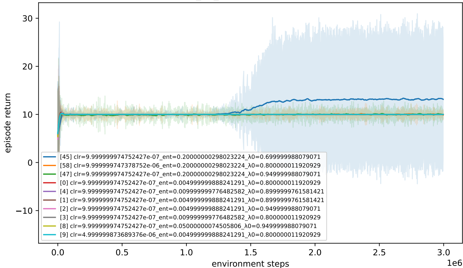
legurnn — rocksample_11_11 (combined 2 studies) — top 10 of 72
