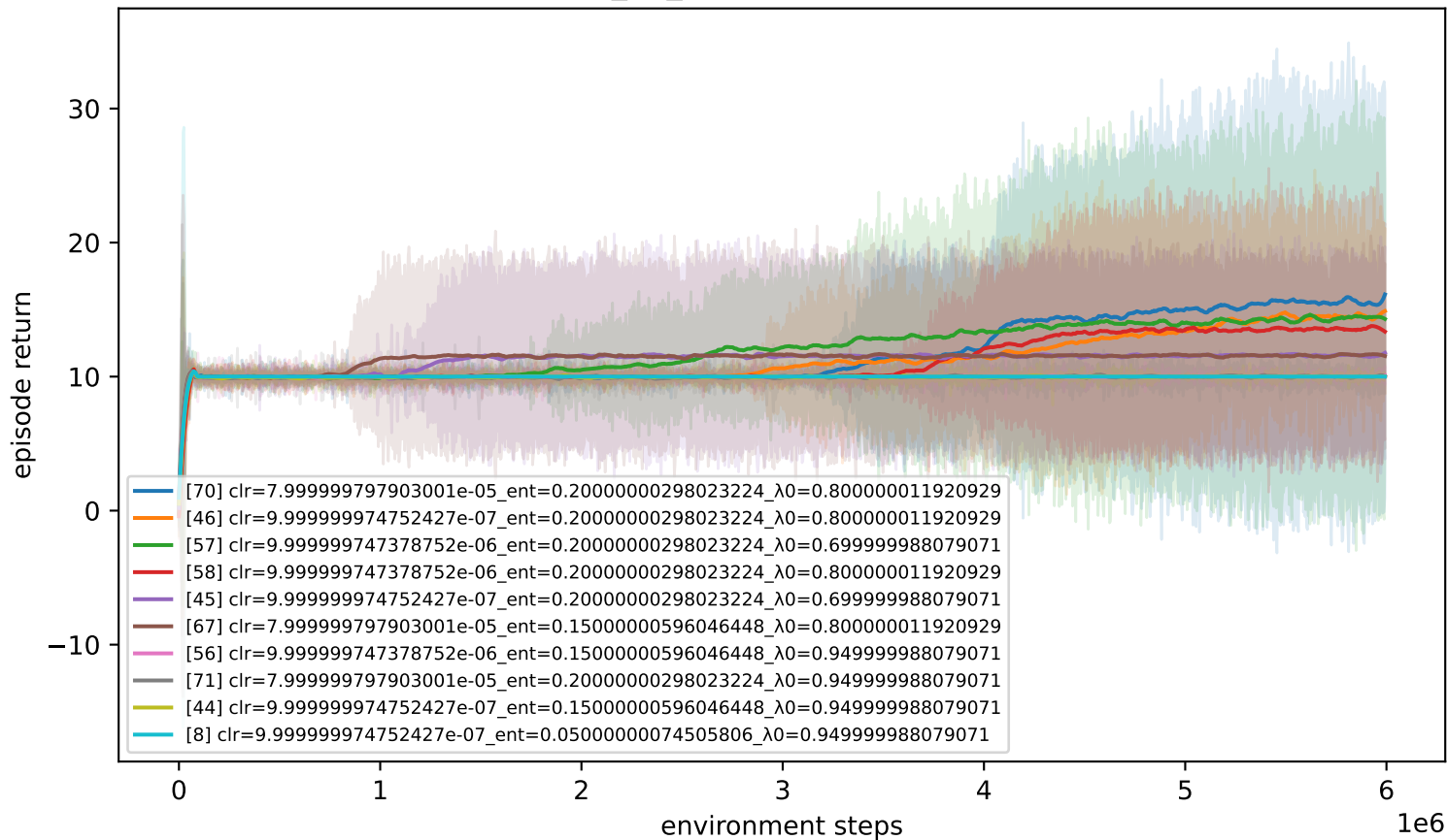
legurnn — rocksample_15_15 (combined 2 studies) — top 10 of 72
