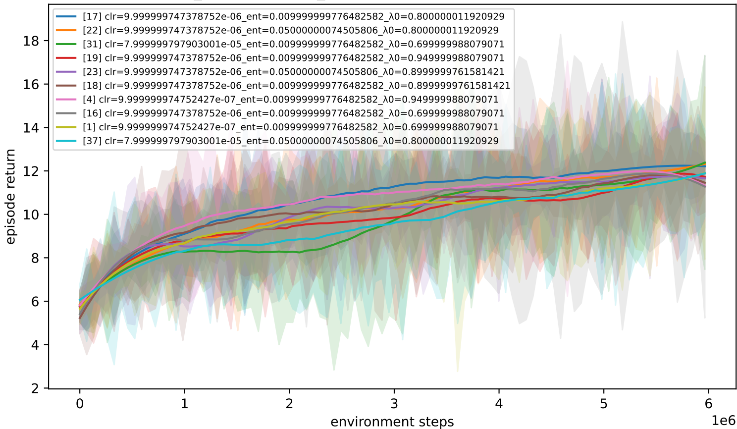
qeunn_2 — battleship_10 (combined 1 studies) — top 10 of 45
