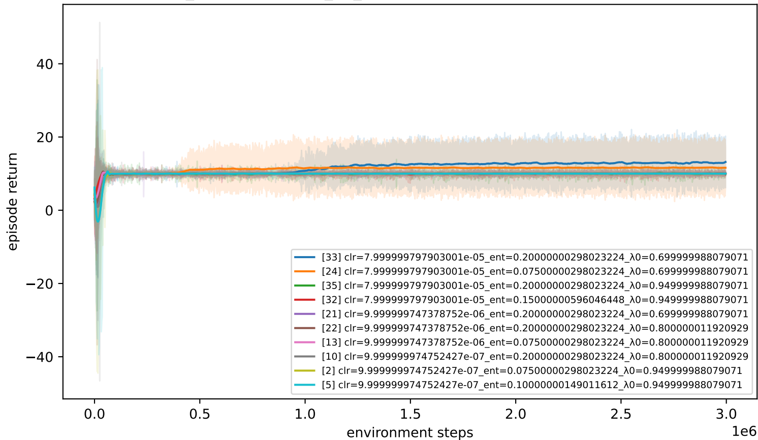
qeunn_2 — rocksample_11_11 (combined 1 studies) — top 10 of 36
