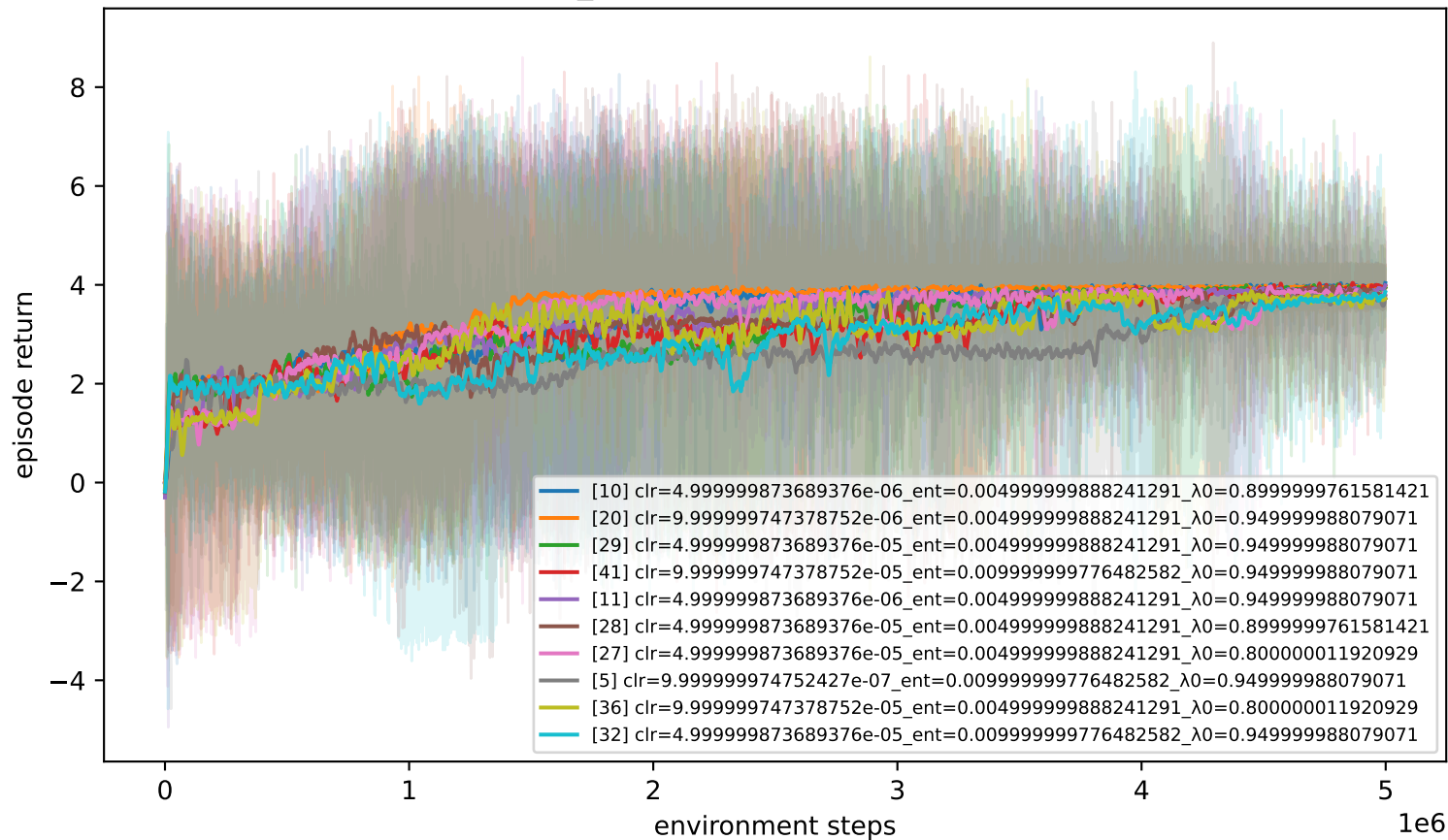
qurnn — tmaze_75 (combined 1 studies) — top 10 of 45
