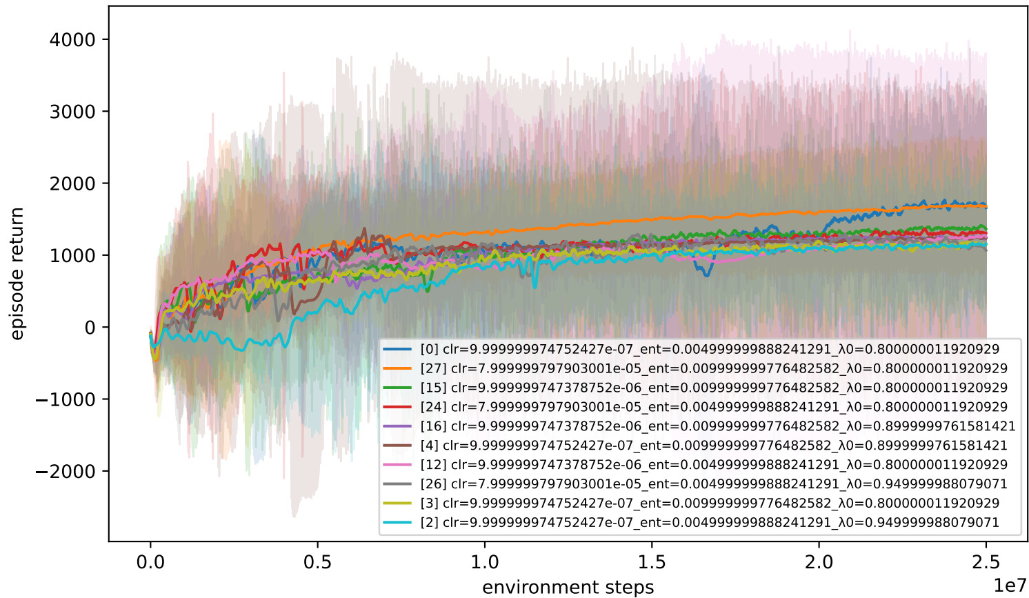
urnn — HalfCheetah-V-v0 (combined 1 studies) — top 10 of 36
