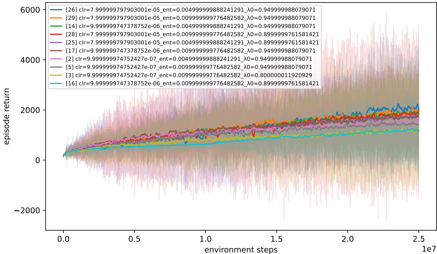
urnn — Walker-V-v0 (combined 1 studies) — top 10 of 36
