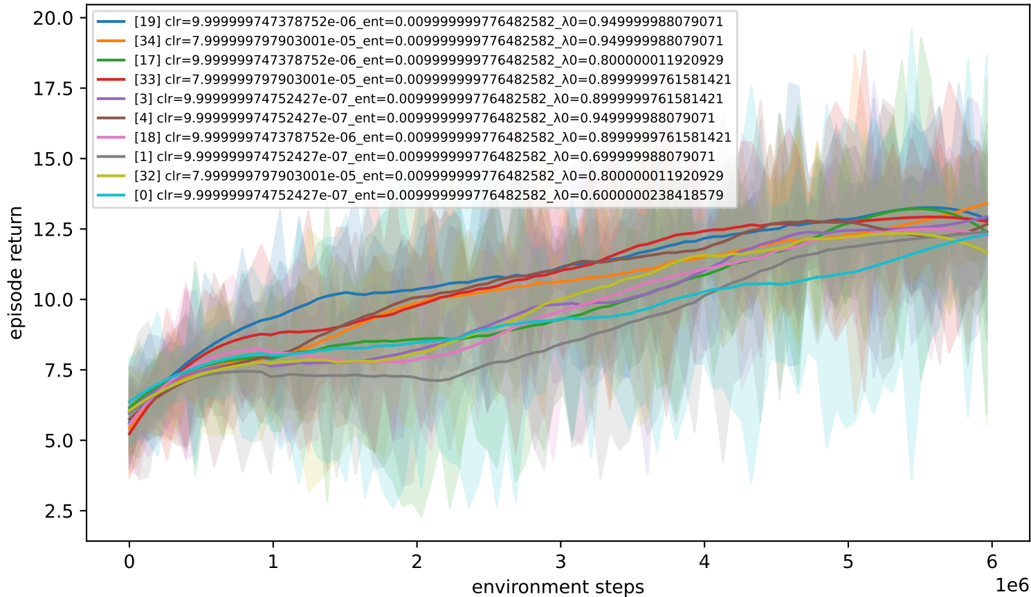
urnn — battleship_10 (combined 1 studies) — top 10 of 45
