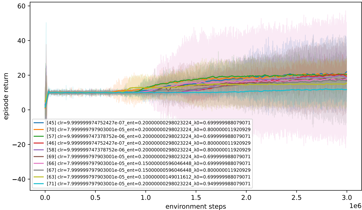
urnn — rocksample_11_11 (combined 2 studies) — top 10 of 72
