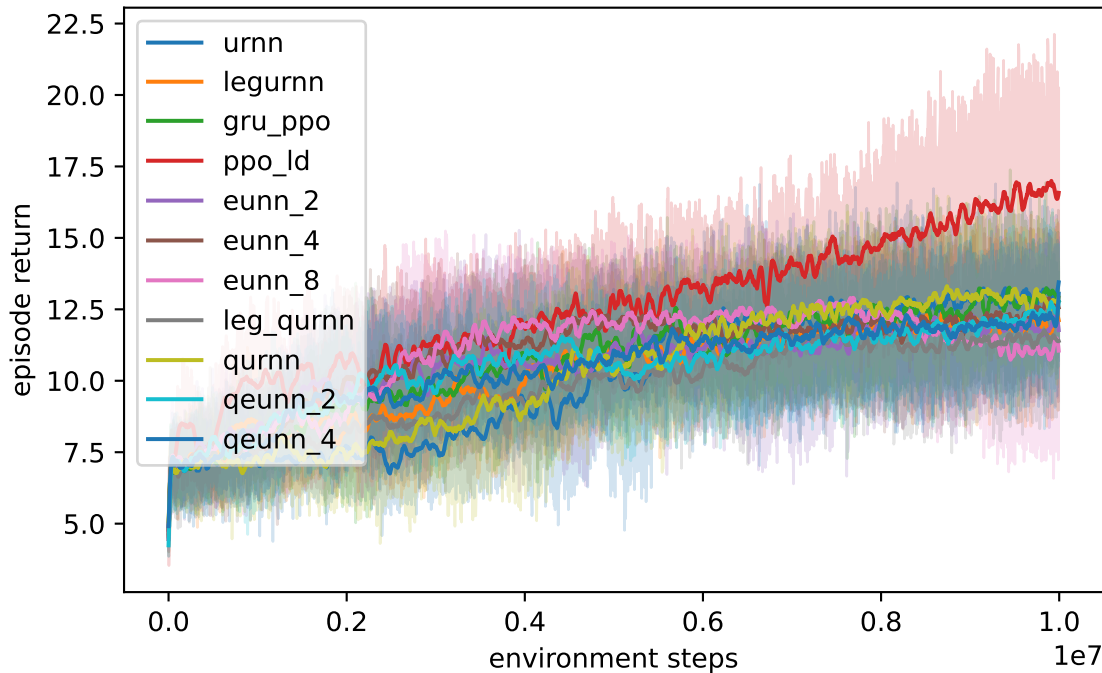
battleship_10
