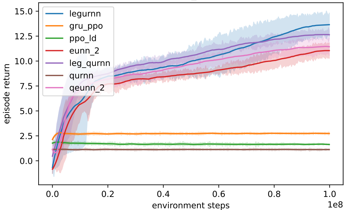
craftax_pixels
