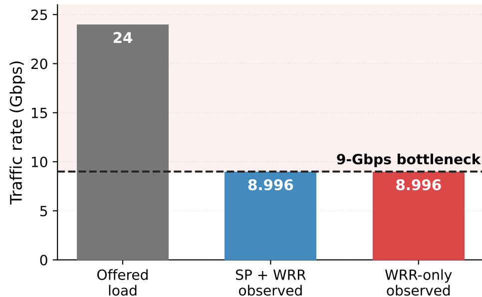
(a) Offered versus observed traffic
