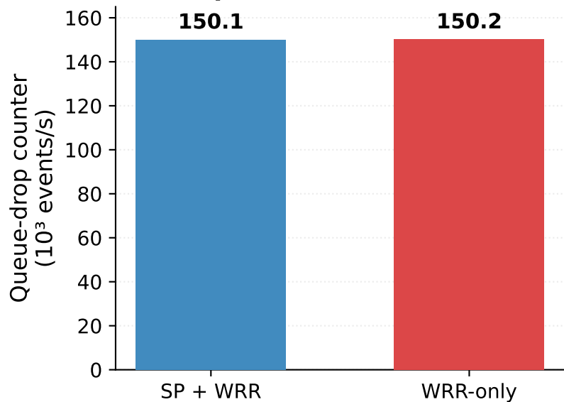
(b) Drops at Router 1
