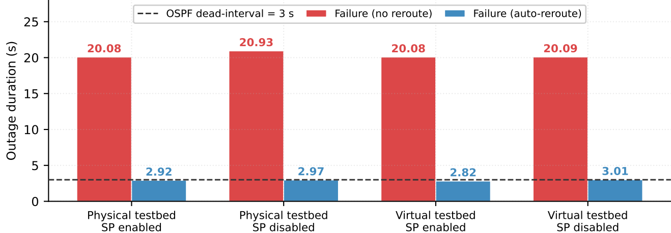
(b) Outage duration across all four conditions
