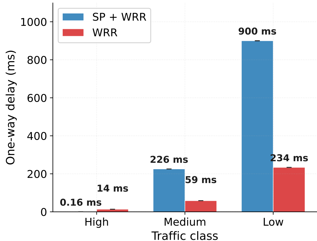
(b) Per-class one-way delay
