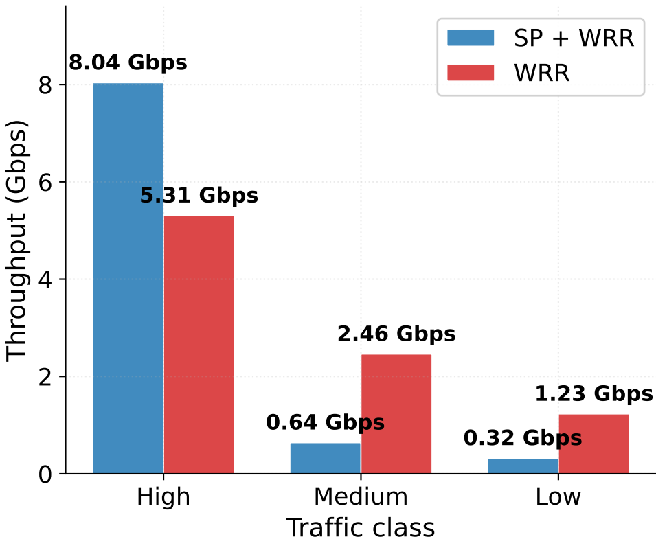
(a) Per-class throughput
